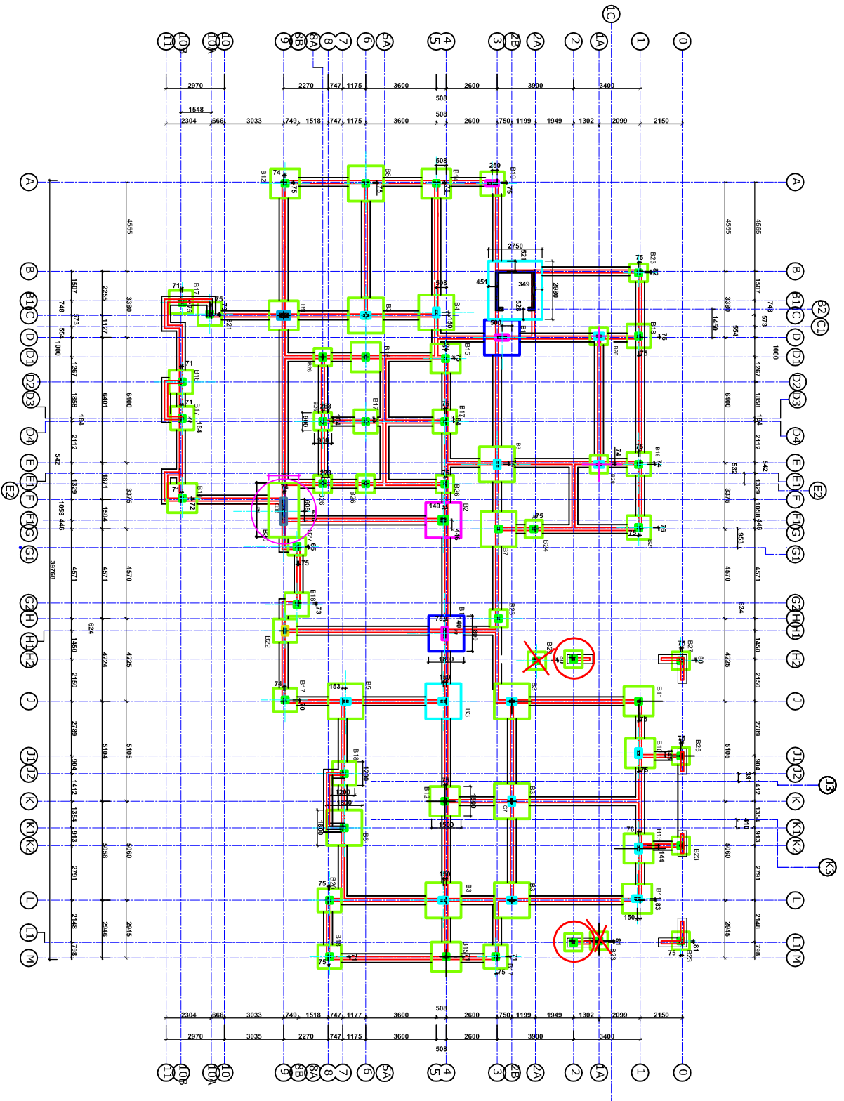
FOUNDATION PLAN
